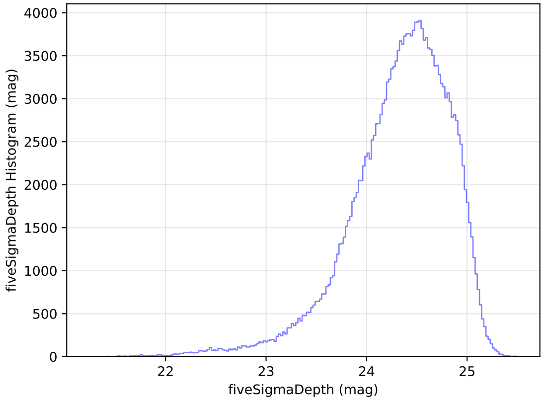
too_elab_r32_d3_giz_v3.4_10yrs All sky g band: fiveSigmaDepth Histogram
