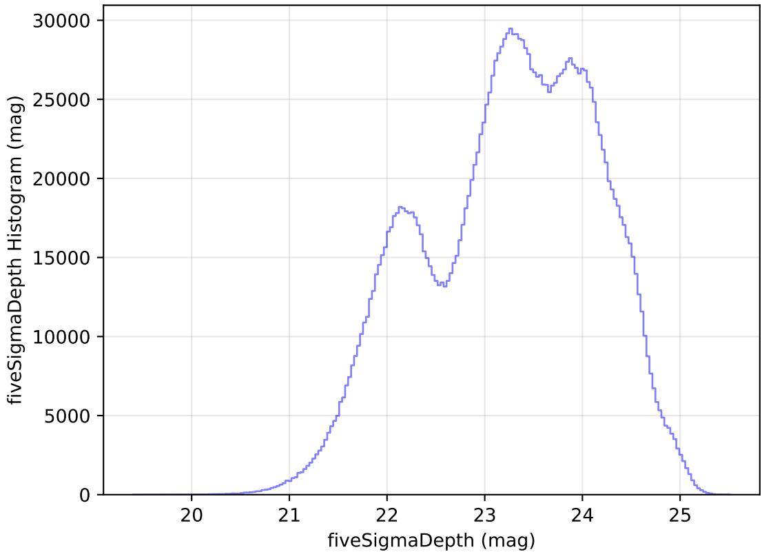
too_elab_r32_d3_giz_v3.4_10yrs All sky all bands: fiveSigmaDepth Histogram
