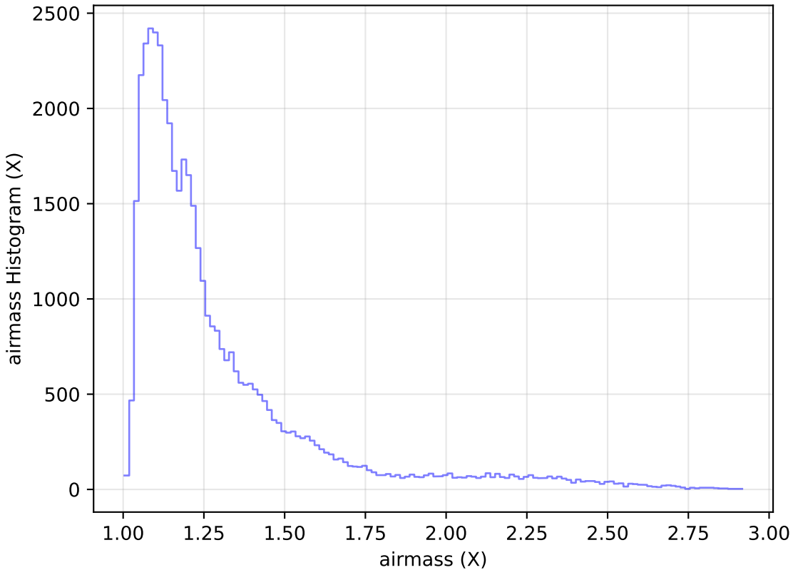
too_elab_r32_d3_giz_v3.4_10yrs Yr 1 z band: airmass Histogram
