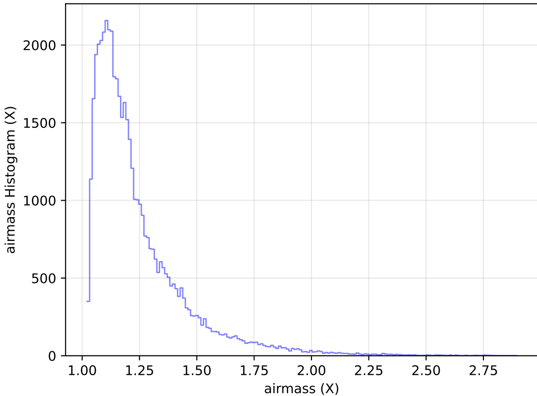
too_elab_r32_d3_giz_v3.4_10yrs Yr 1 y band: airmass Histogram
