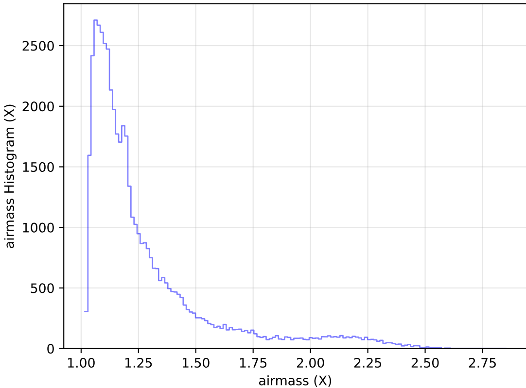
too_elab_r32_d3_giz_v3.4_10yrs Yr 1 r band: airmass Histogram
