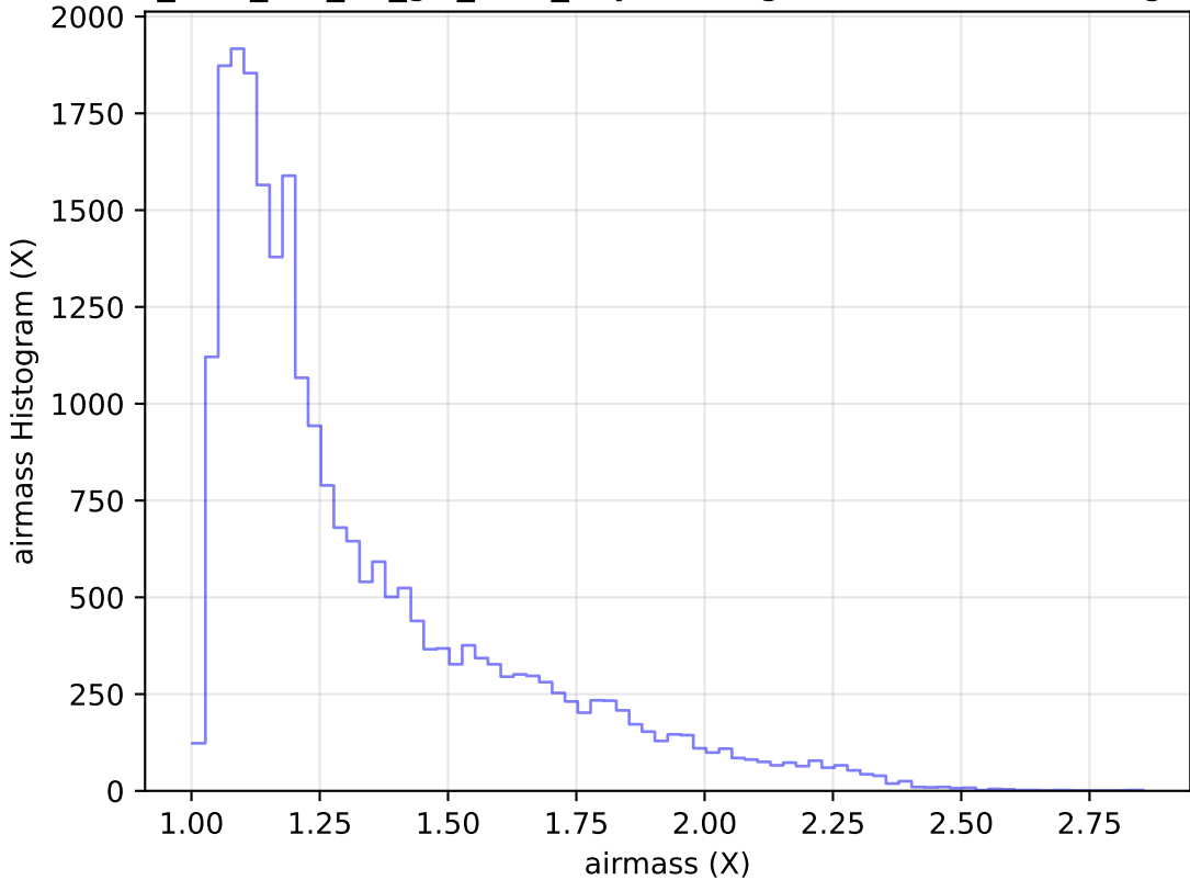
too_elab_r32_d3_giz_v3.4_10yrs Yr 1 g band: airmass Histogram
