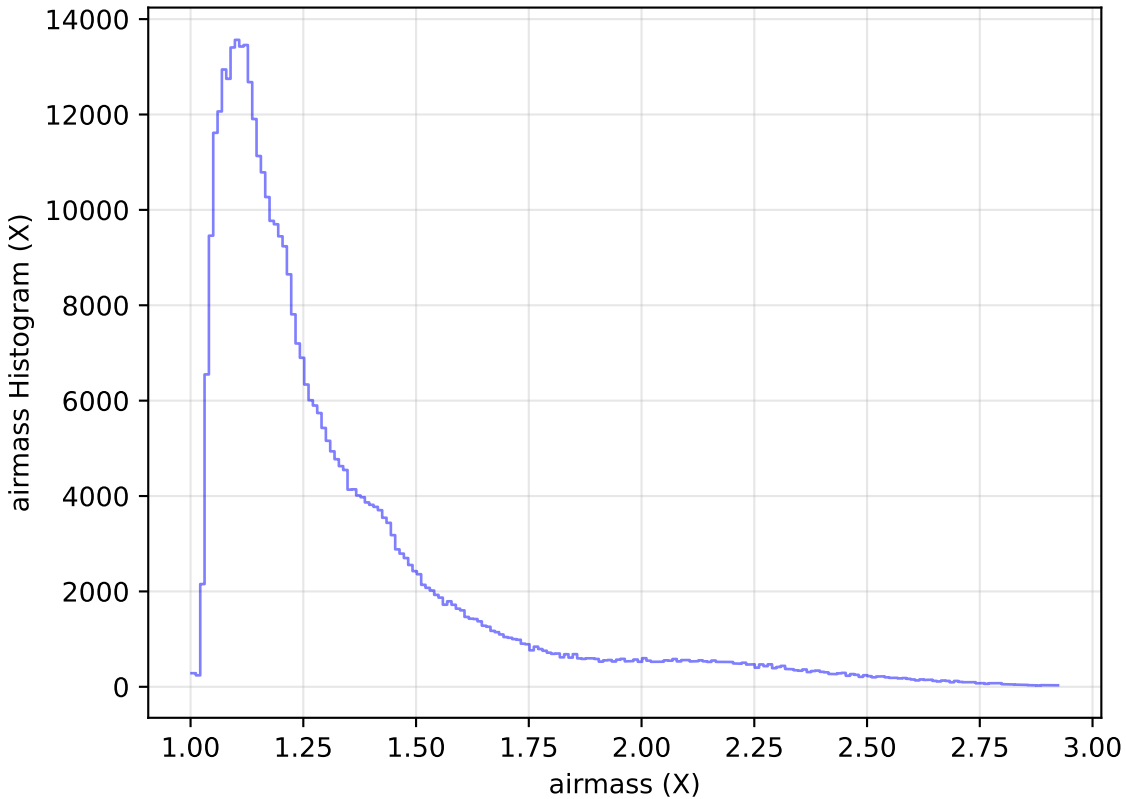
too_elab_r32_d3_giz_v3.4_10yrs WFD z band: airmass Histogram
