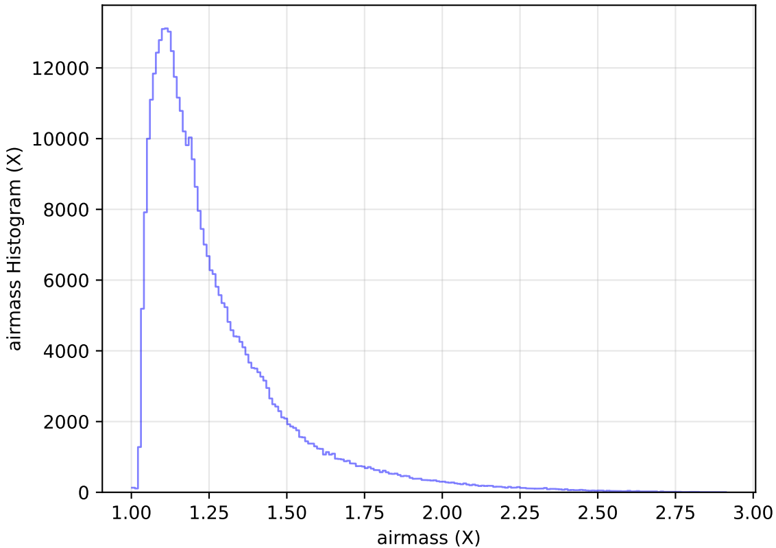
too_elab_r32_d3_giz_v3.4_10yrs WFD y band: airmass Histogram
