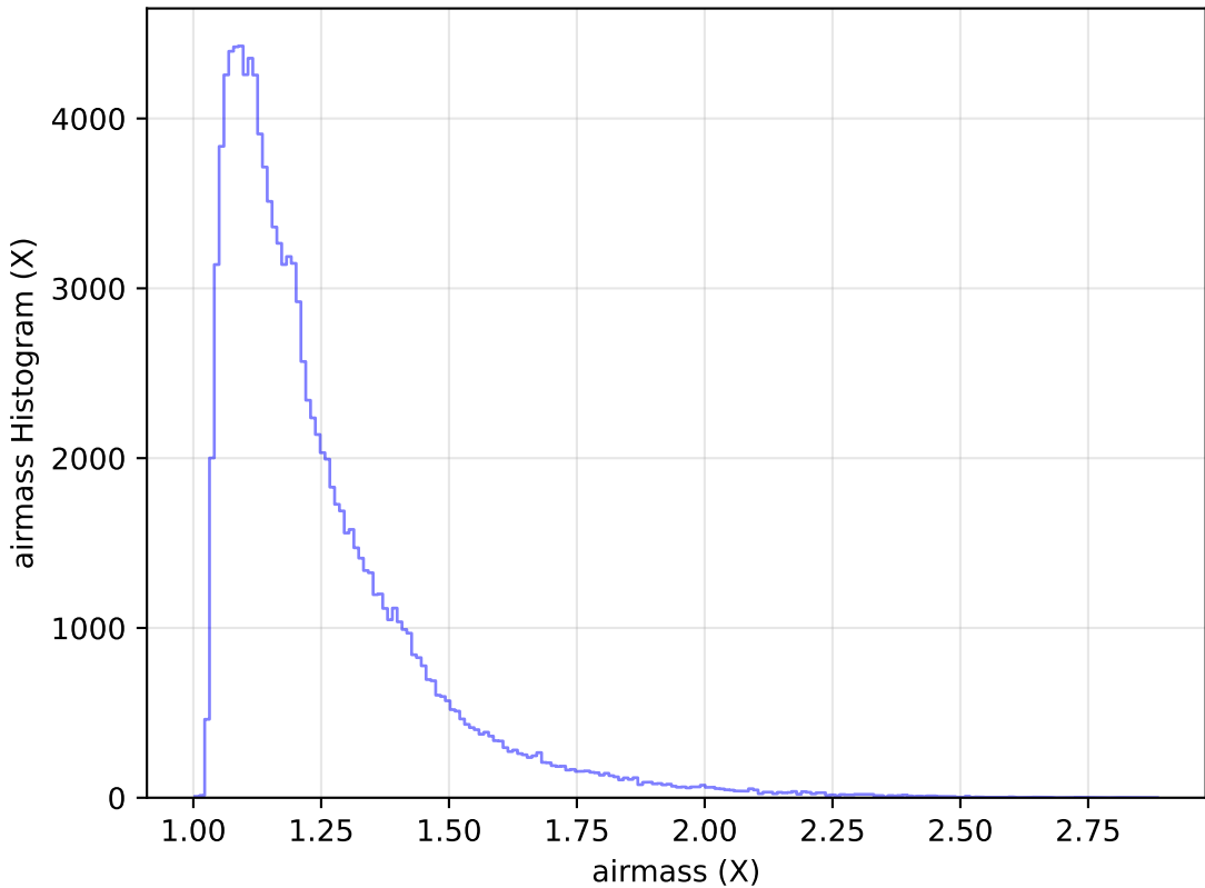
too_elab_r32_d3_giz_v3.4_10yrs WFD u band: airmass Histogram
