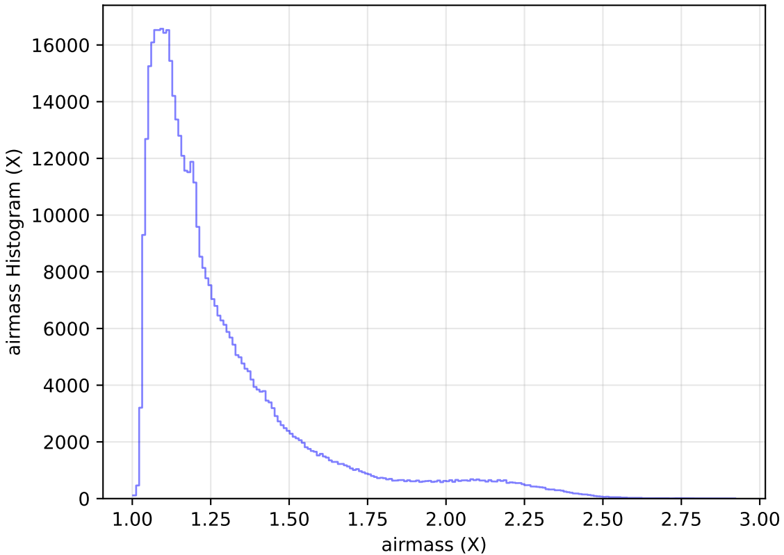
too_elab_r32_d3_giz_v3.4_10yrs WFD r band: airmass Histogram
