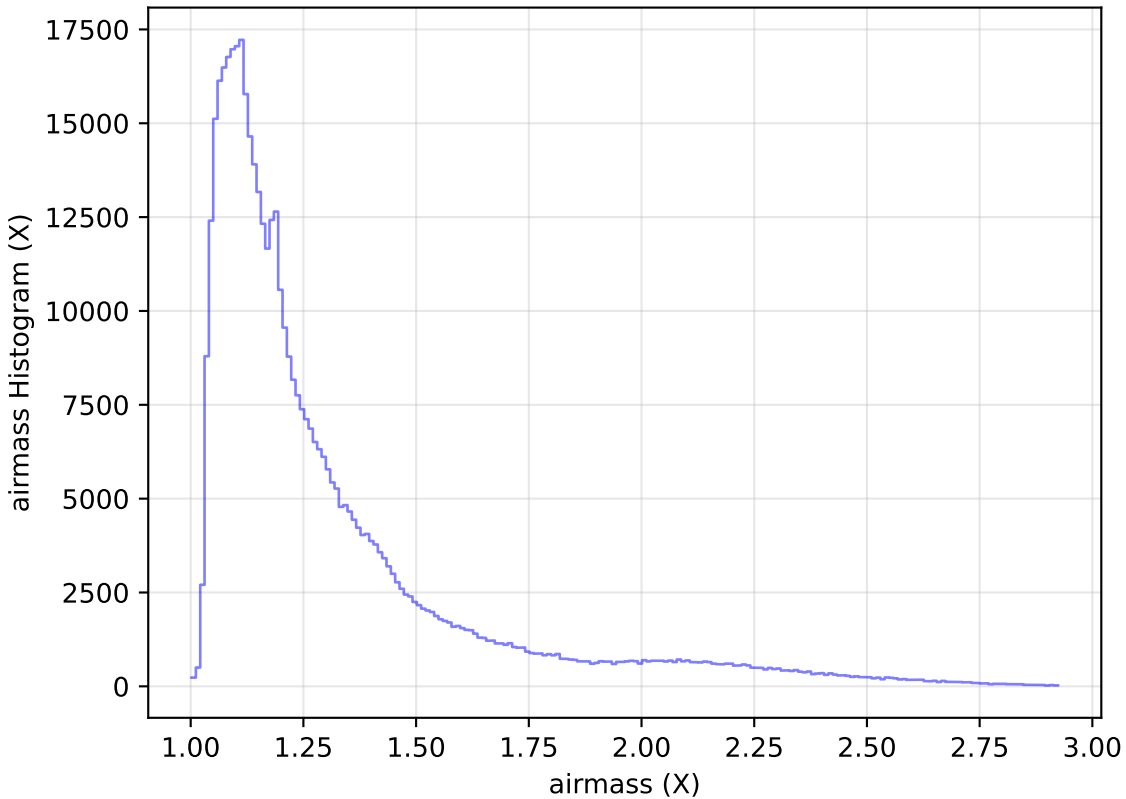
too_elab_r32_d3_giz_v3.4_10yrs WFD i band: airmass Histogram
