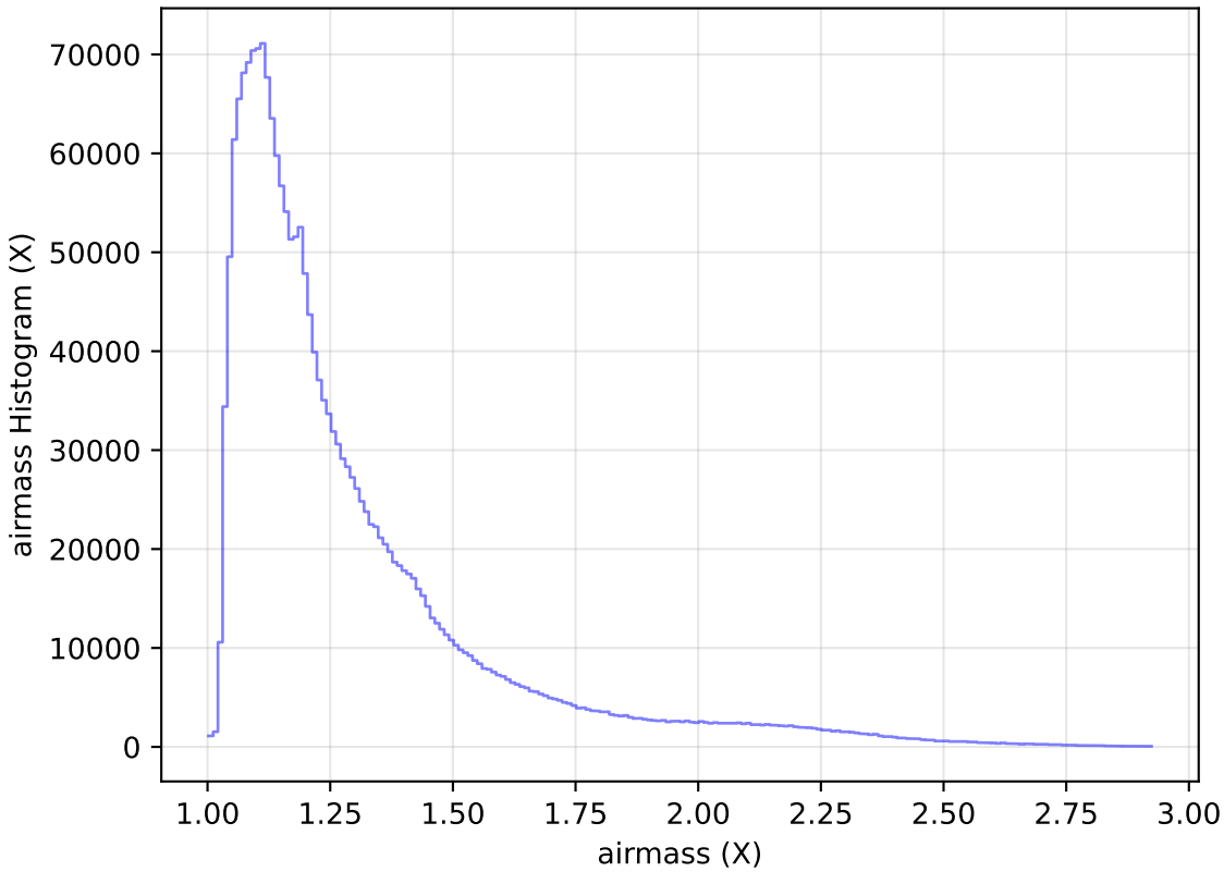
too_elab_r32_d3_giz_v3.4_10yrs WFD all bands: airmass Histogram
