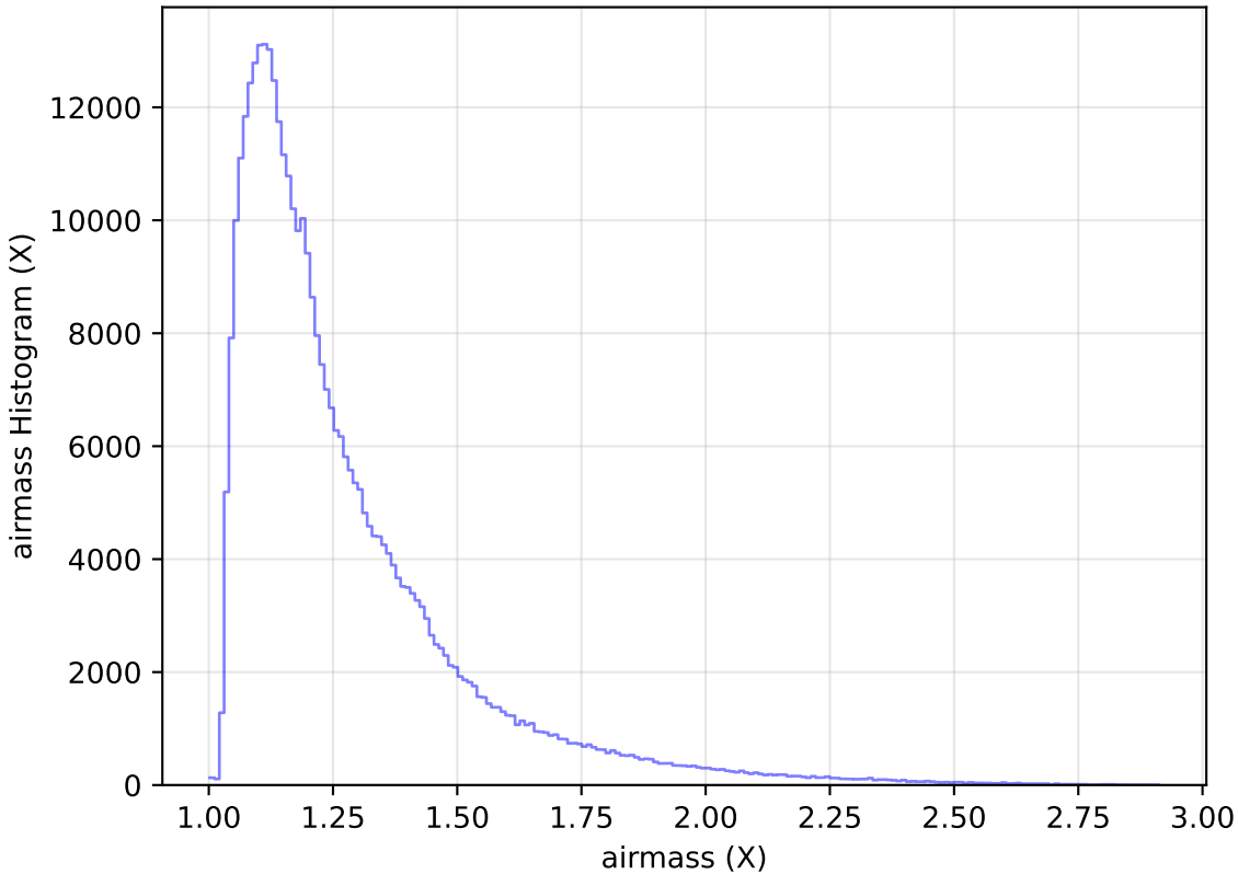
too_elab_r32_d3_giz_v3.4_10yrs All sky y band: airmass Histogram
