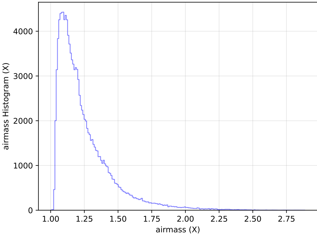
too_elab_r32_d3_giz_v3.4_10yrs All sky u band: airmass Histogram
