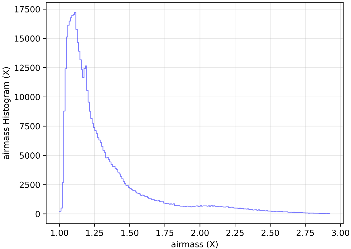
too_elab_r32_d3_giz_v3.4_10yrs All sky i band: airmass Histogram
