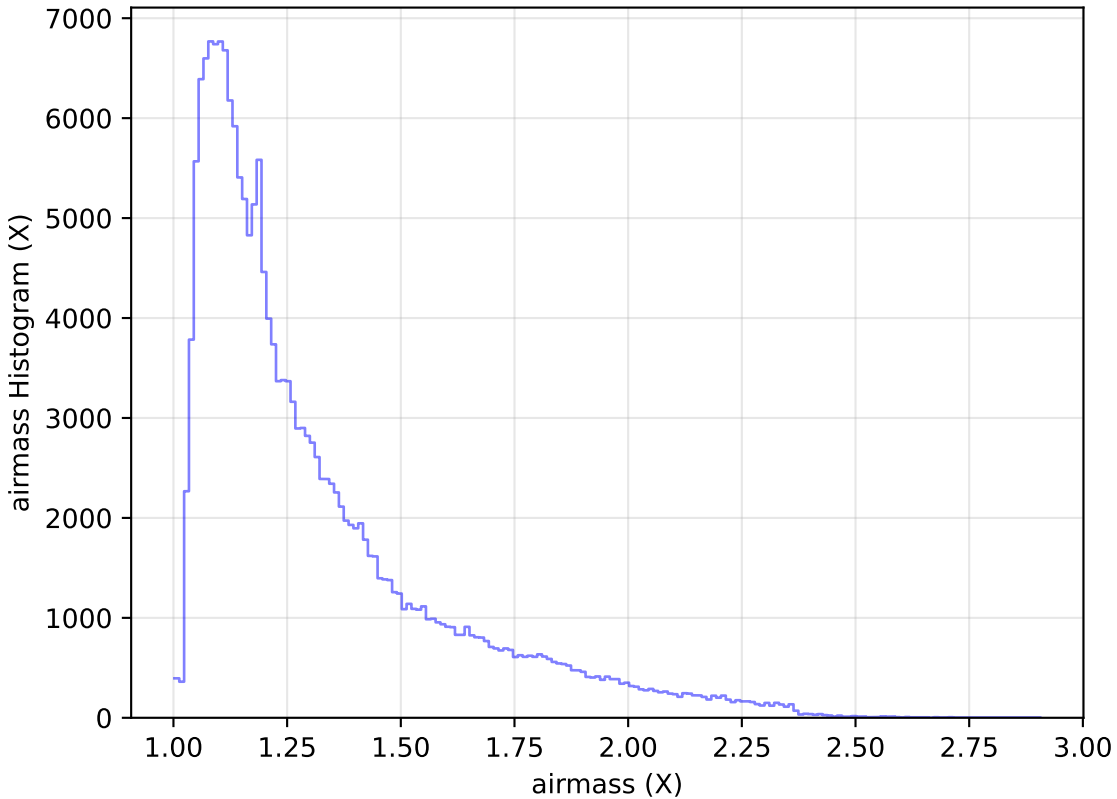
too_elab_r32_d3_giz_v3.4_10yrs All sky g band: airmass Histogram
