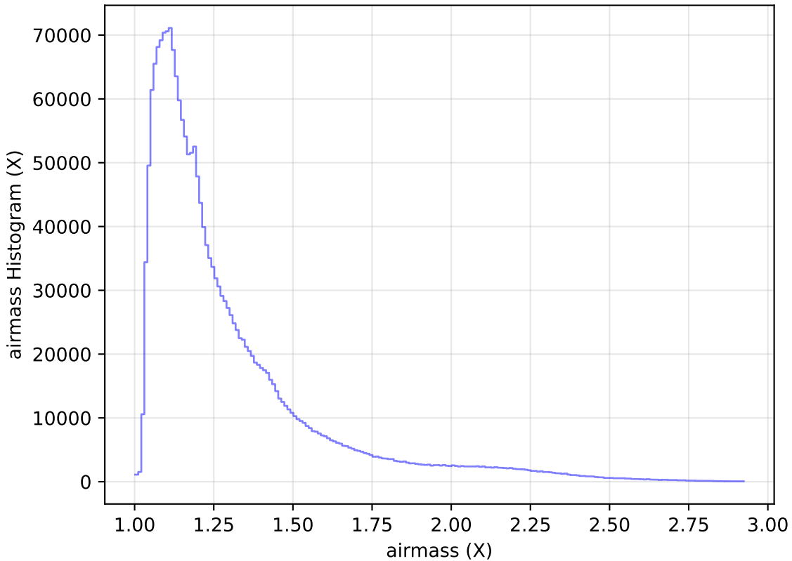
too_elab_r32_d3_giz_v3.4_10yrs All sky all bands: airmass Histogram
