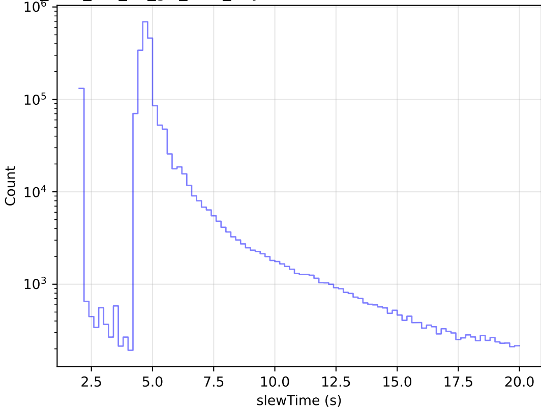
too_elab_r32_d3_giz_v3.4_10yrs All visits: Zoom Slew Time Histogram
