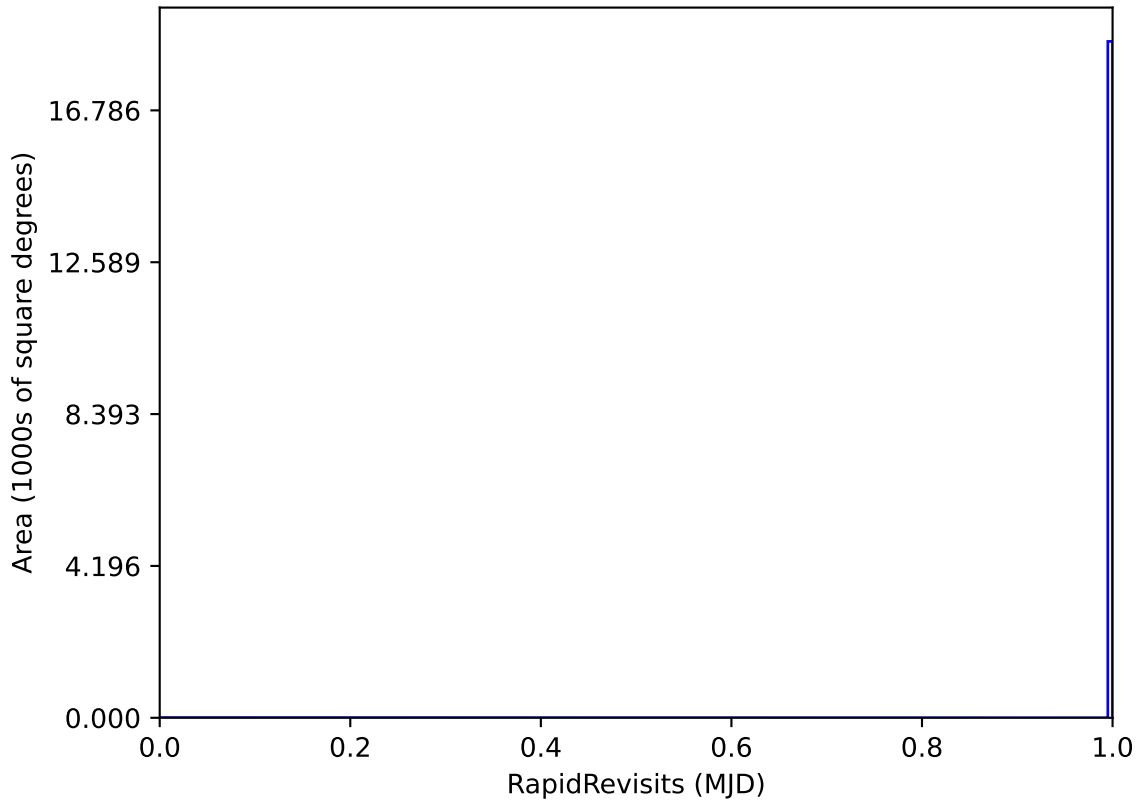
too_elab_r32_d3_giz_v3.4_10yrs WFD: RapidRevisits
