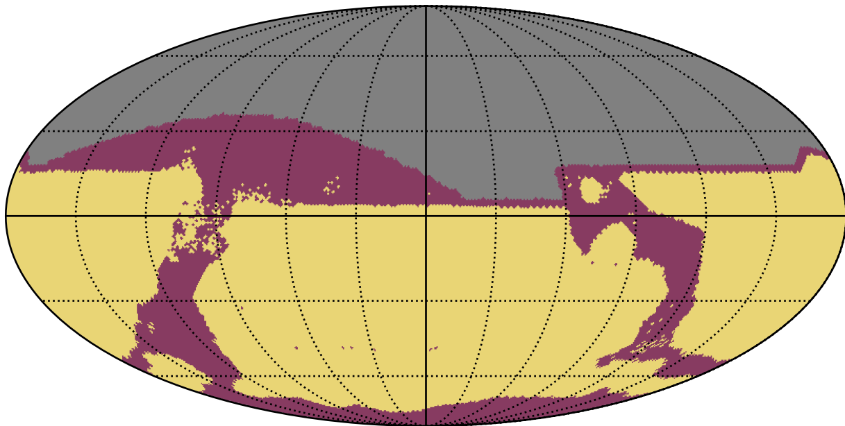
too_elab_r32_d3_giz_v3.4_10yrs All sky: RapidRevisits
