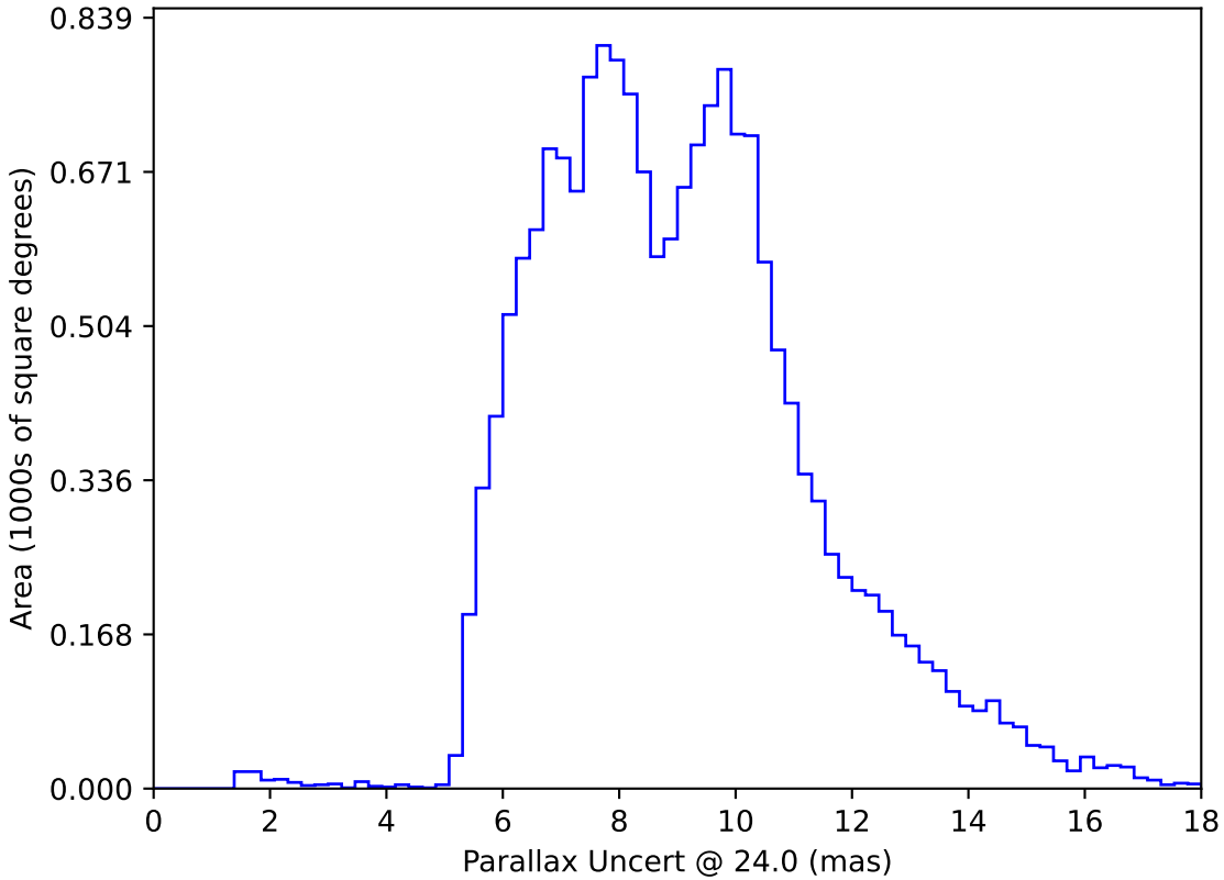
too_elab_r32_d3_giz_v3.4_10yrs WFD: Parallax Uncert @ 24.0
