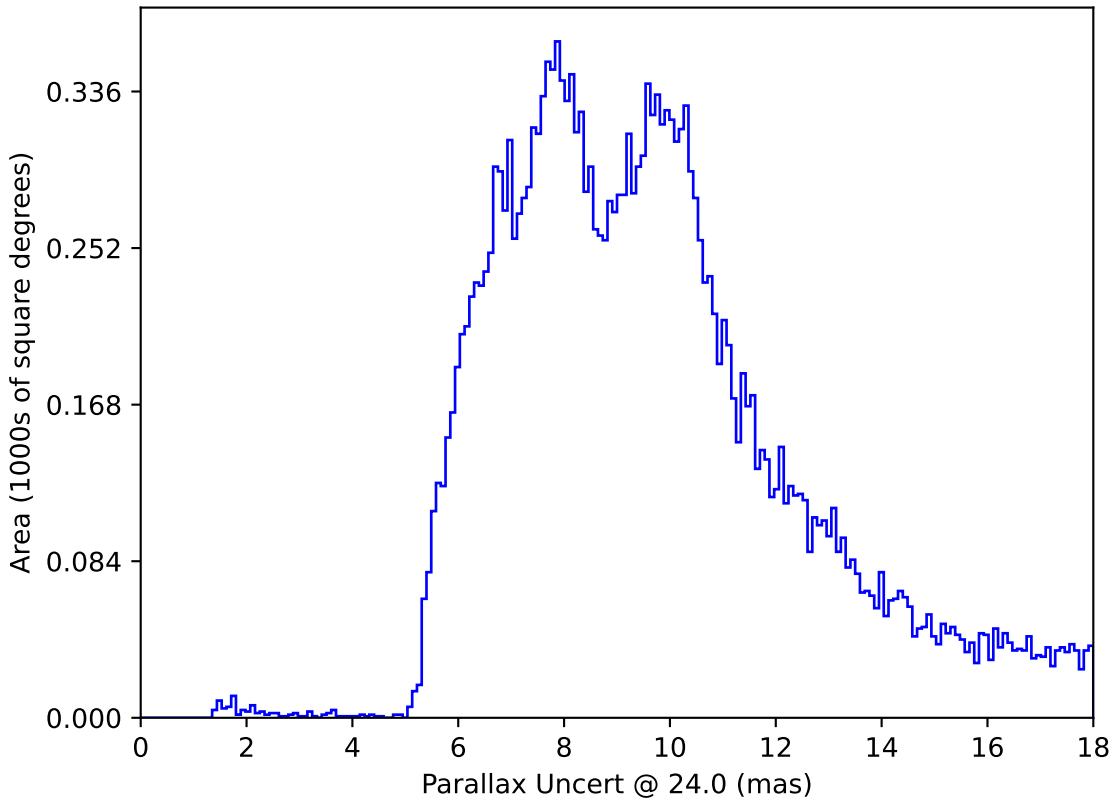
too_elab_r32_d3_giz_v3.4_10yrs All sky: Parallax Uncert @ 24.0
