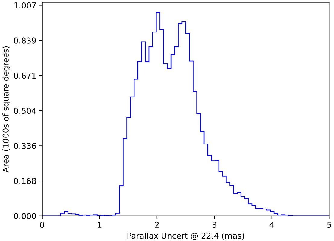
too_elab_r32_d3_giz_v3.4_10yrs WFD: Parallax Uncert @ 22.4
