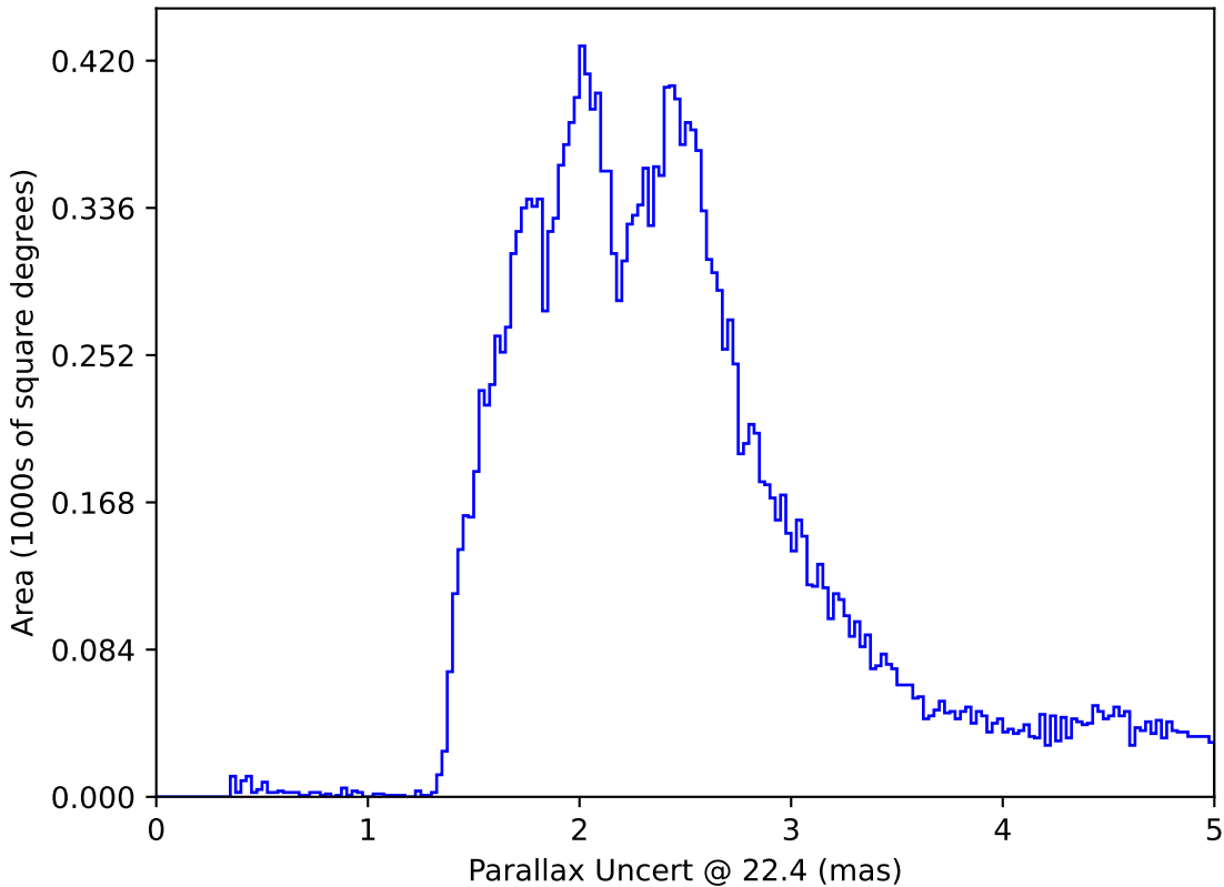
too_elab_r32_d3_giz_v3.4_10yrs All sky: Parallax Uncert @ 22.4
