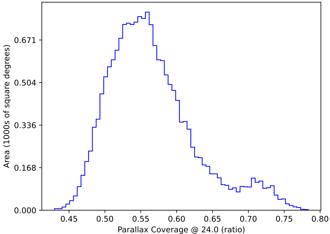
too_elab_r32_d3_giz_v3.4_10yrs WFD: Parallax Coverage @ 24.0
