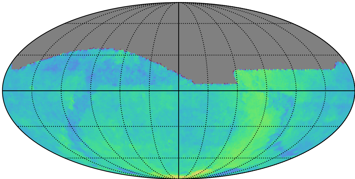
too_elab_r32_d3_giz_v3.4_10yrs All sky: Parallax Coverage @ 24.0
