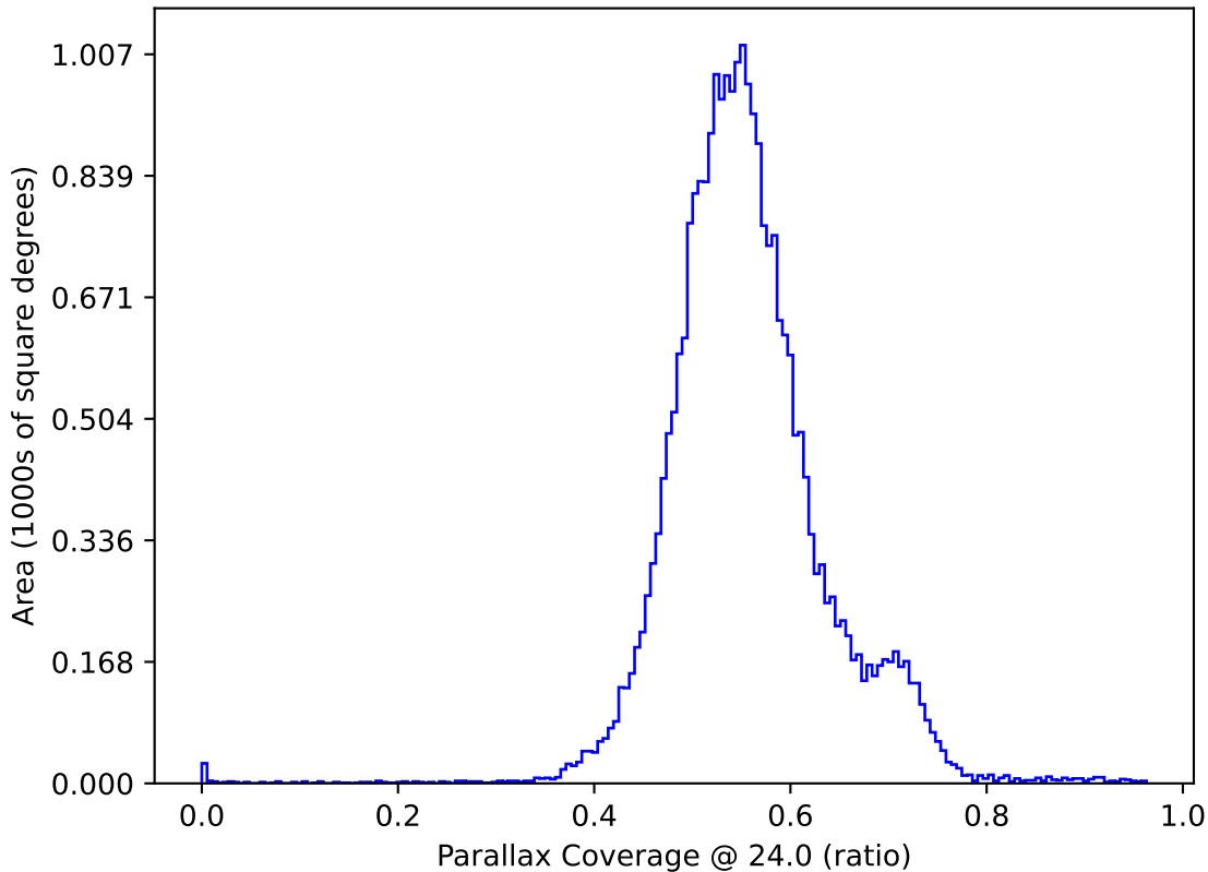
too_elab_r32_d3_giz_v3.4_10yrs All sky: Parallax Coverage @ 24.0
