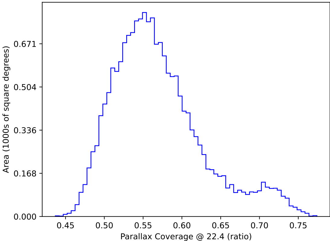
too_elab_r32_d3_giz_v3.4_10yrs WFD: Parallax Coverage @ 22.4
