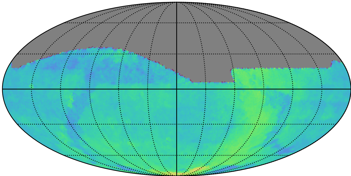
too_elab_r32_d3_giz_v3.4_10yrs All sky: Parallax Coverage @ 22.4
