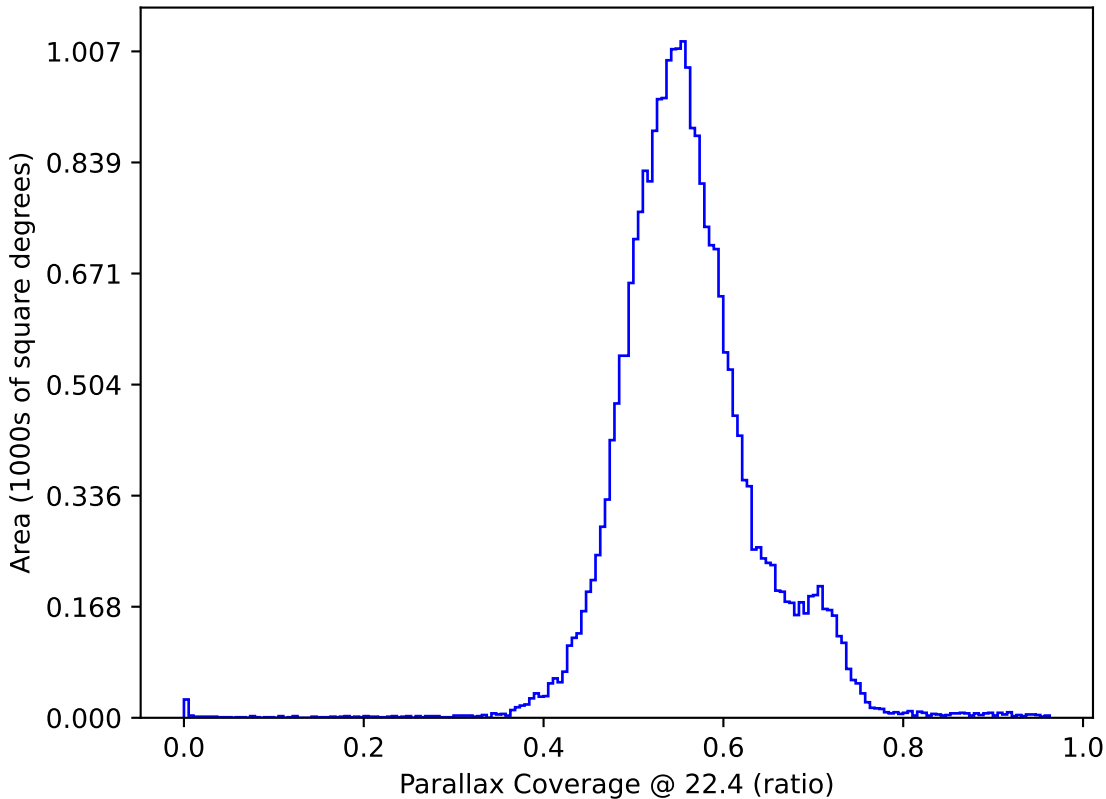
too_elab_r32_d3_giz_v3.4_10yrs All sky: Parallax Coverage @ 22.4
