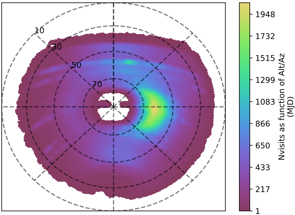
too_elab_r32_d3_giz_v3.4_10yrs y band: Nvisits as function of Alt/Az
