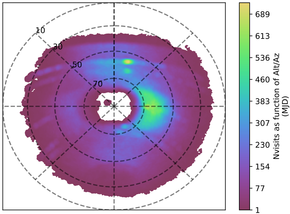
too_elab_r32_d3_giz_v3.4_10yrs u band: Nvisits as function of Alt/Az
