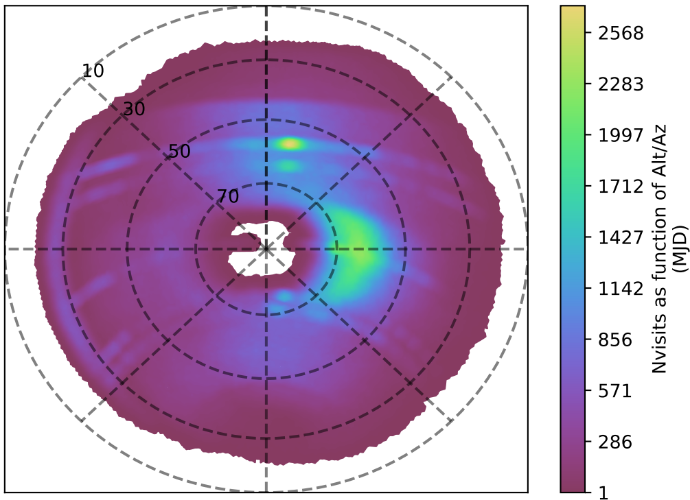
too_elab_r32_d3_giz_v3.4_10yrs r band: Nvisits as function of Alt/Az
