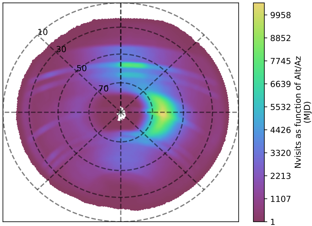
too_elab_r32_d3_giz_v3.4_10yrs all bands: Nvisits as function of Alt/Az
