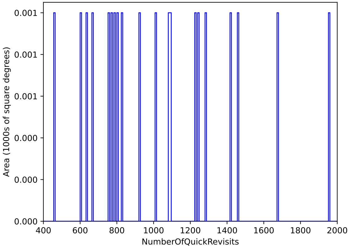
too_elab_r32_d3_giz_v3.4_10yrs WFD: NumberOfQuickRevisits
