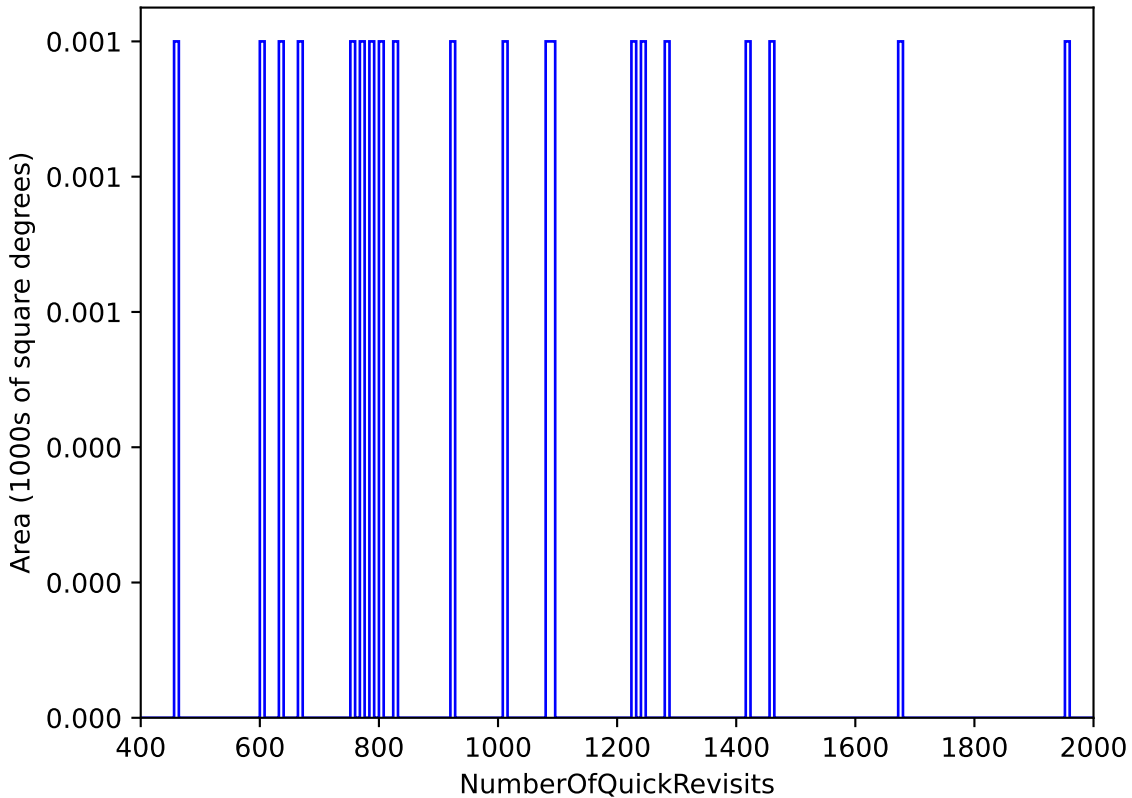
too_elab_r32_d3_giz_v3.4_10yrs All sky: NumberOfQuickRevisits
