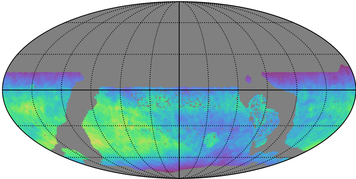
too_elab_r32_d3_giz_v3.4_10yrs WFD z band: Normalized Teff
