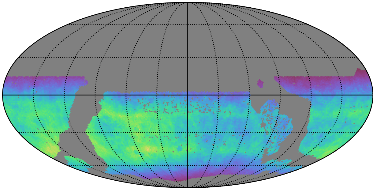
too_elab_r32_d3_giz_v3.4_10yrs WFD y band: Normalized Teff
