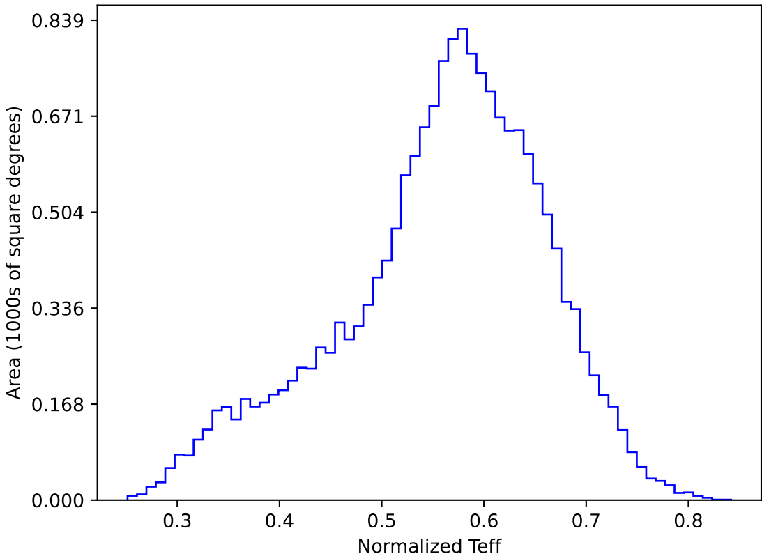
too_elab_r32_d3_giz_v3.4_10yrs WFD y band: Normalized Teff
