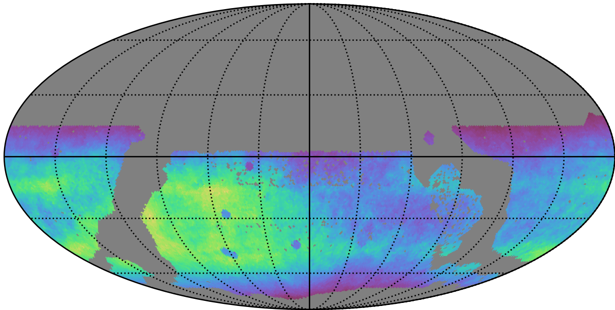
too_elab_r32_d3_giz_v3.4_10yrs WFD r band: Normalized Teff
