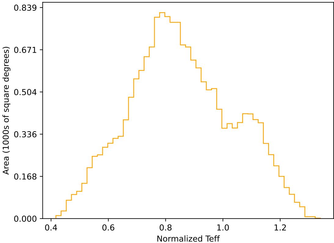
too_elab_r32_d3_giz_v3.4_10yrs WFD r band: Normalized Teff
