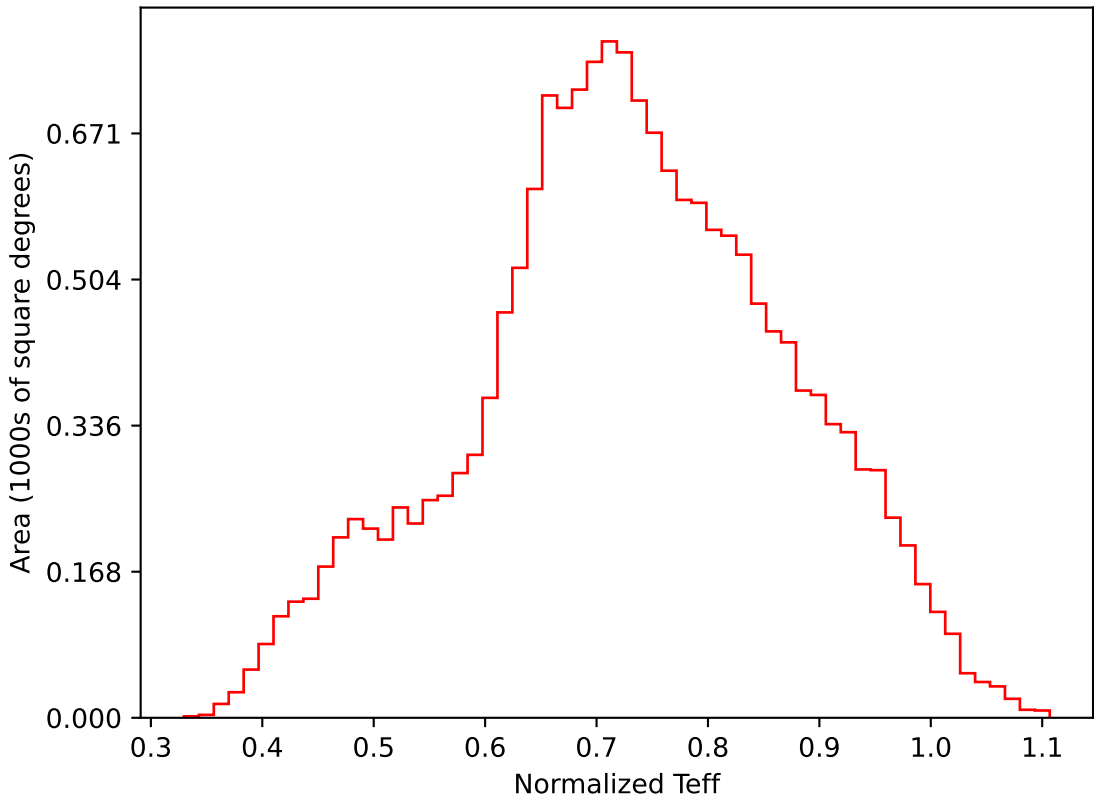
too_elab_r32_d3_giz_v3.4_10yrs WFD i band: Normalized Teff
