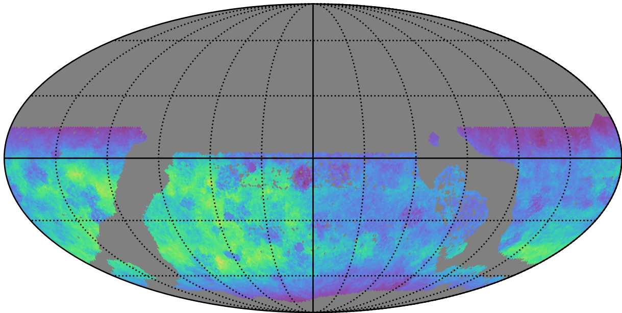
too_elab_r32_d3_giz_v3.4_10yrs WFD g band: Normalized Teff
