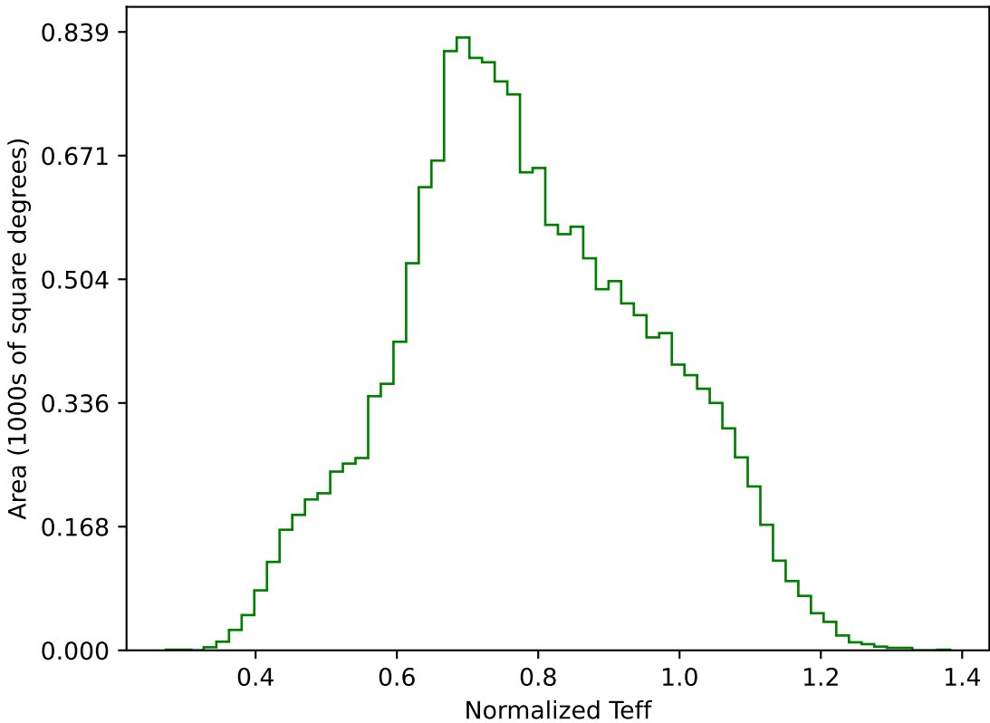
too_elab_r32_d3_giz_v3.4_10yrs WFD g band: Normalized Teff
