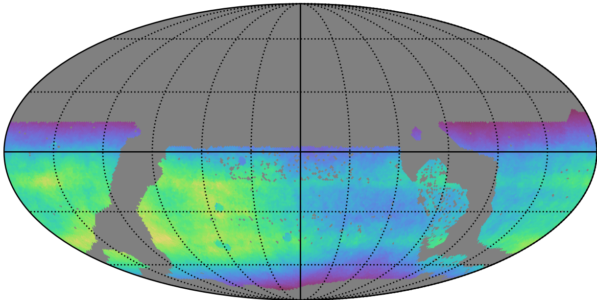
too_elab_r32_d3_giz_v3.4_10yrs WFD all bands: Normalized Teff
