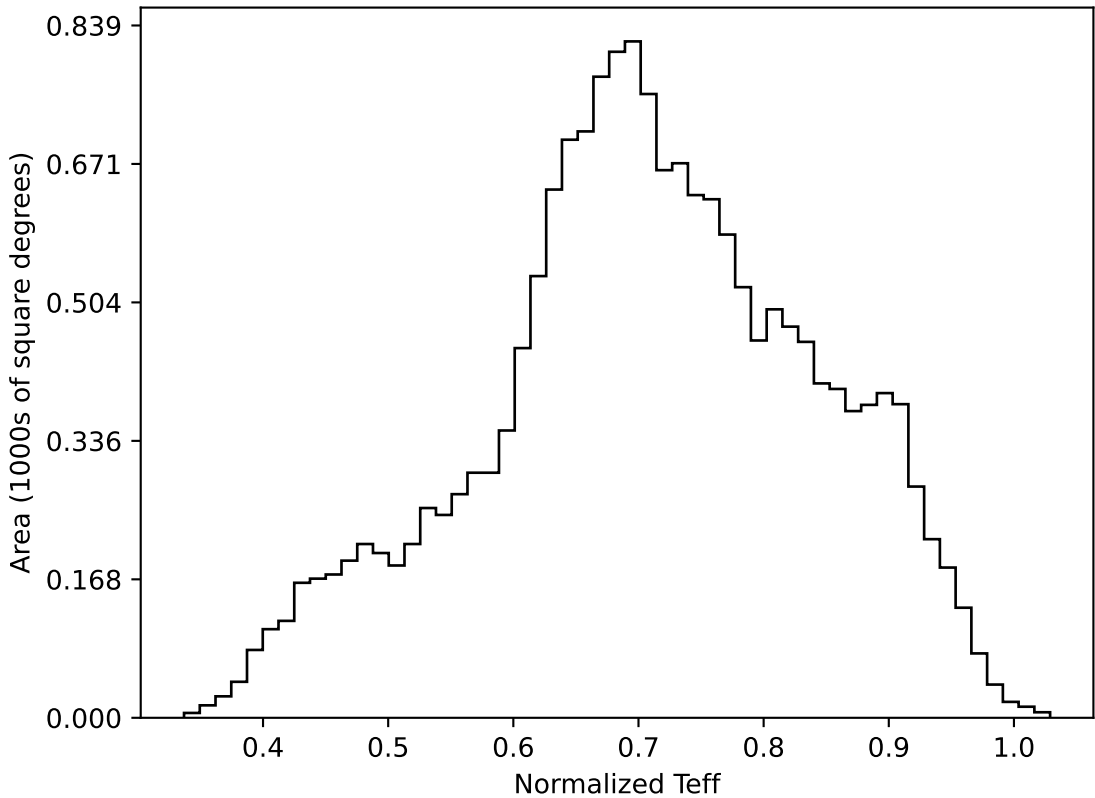
too_elab_r32_d3_giz_v3.4_10yrs WFD all bands: Normalized Teff
