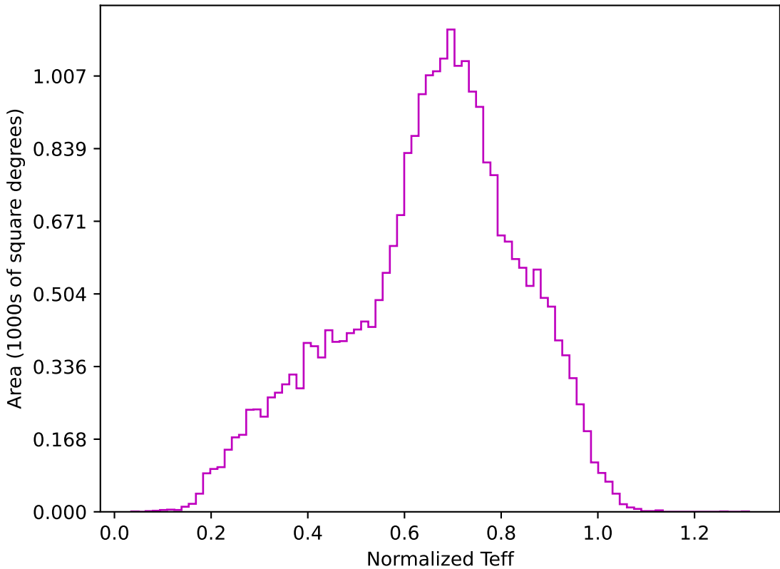
too_elab_r32_d3_giz_v3.4_10yrs All sky z band: Normalized Teff
