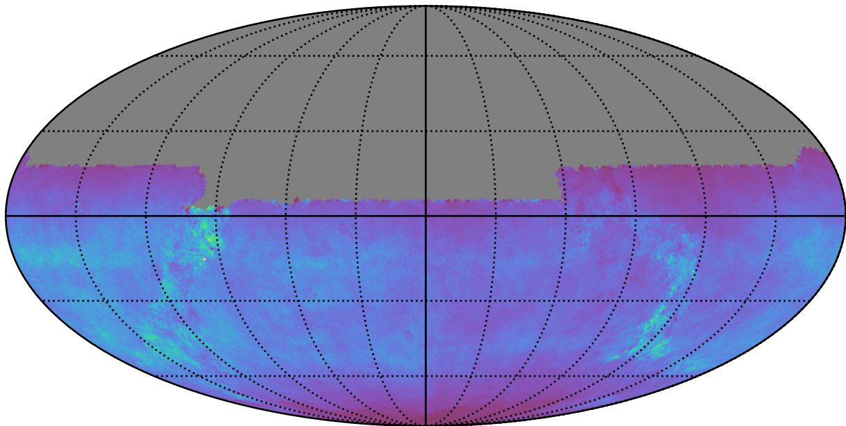
too_elab_r32_d3_giz_v3.4_10yrs All sky u band: Normalized Teff
