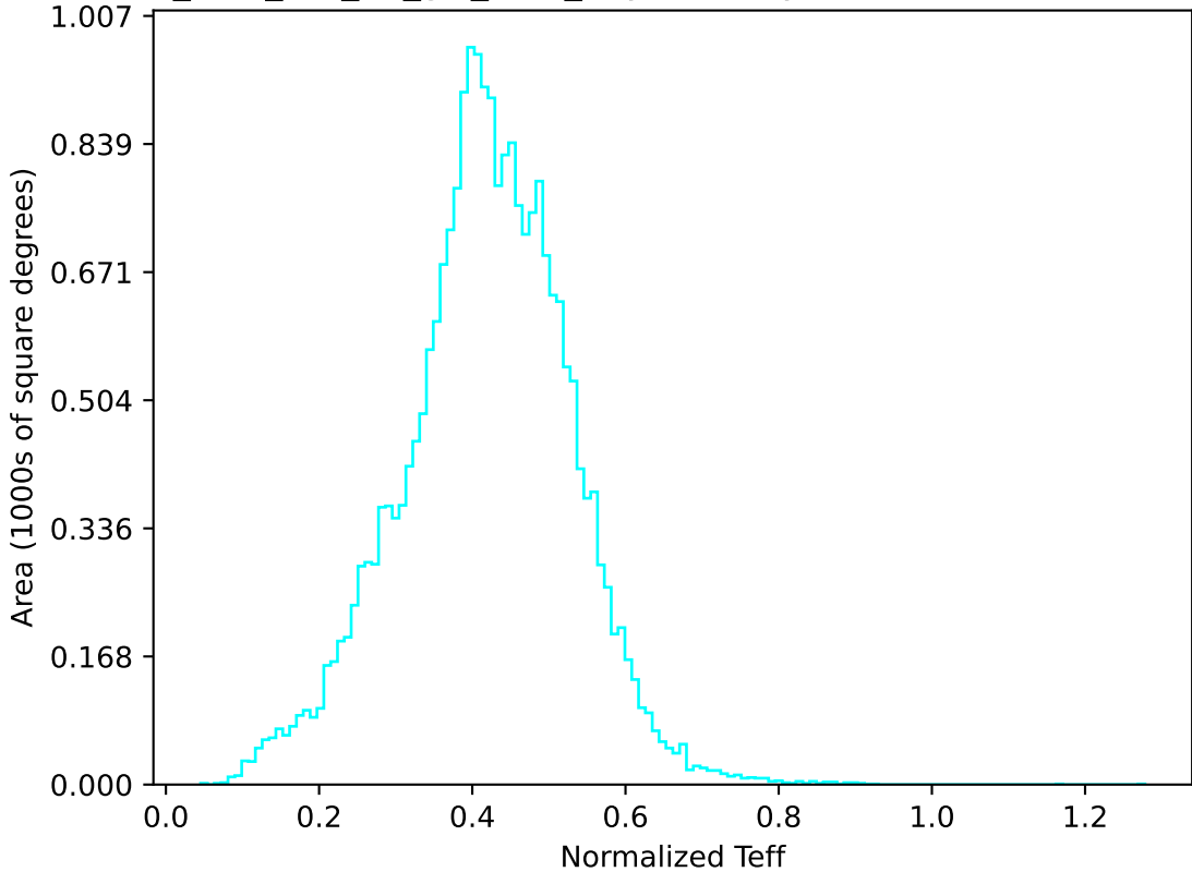
too_elab_r32_d3_giz_v3.4_10yrs All sky u band: Normalized Teff
