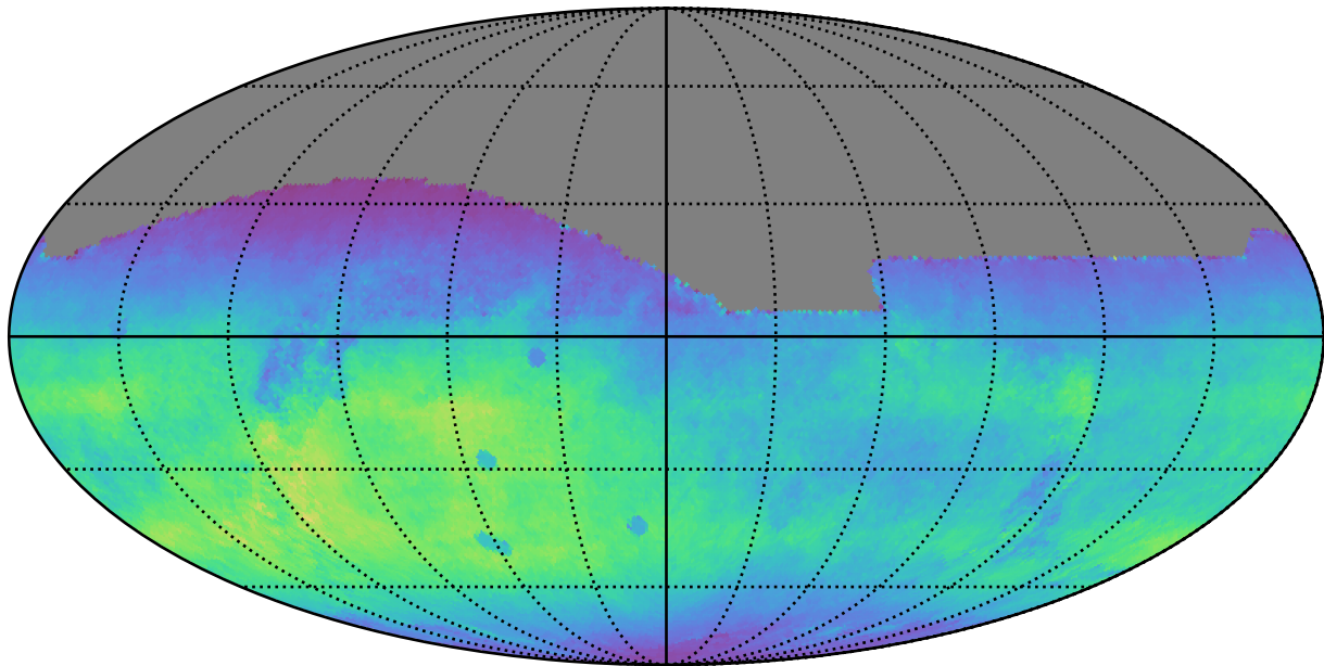
too_elab_r32_d3_giz_v3.4_10yrs All sky r band: Normalized Teff
